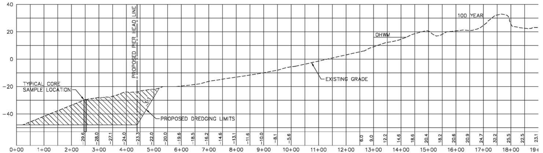
1 C05 CROSS SECTION C-C SCALE: HORZ: 1"=200' VERT: 1"=40'
